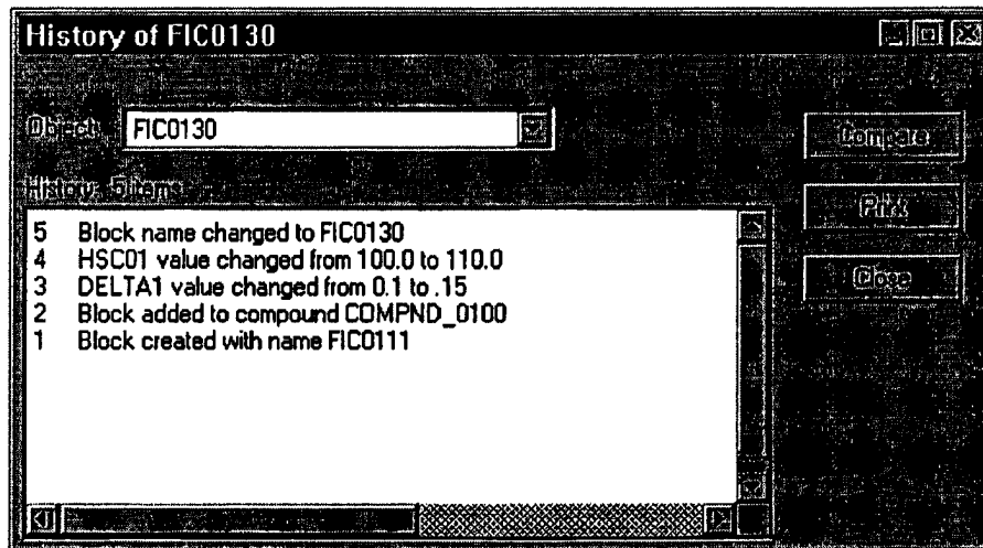
Figure 52 - Version History
